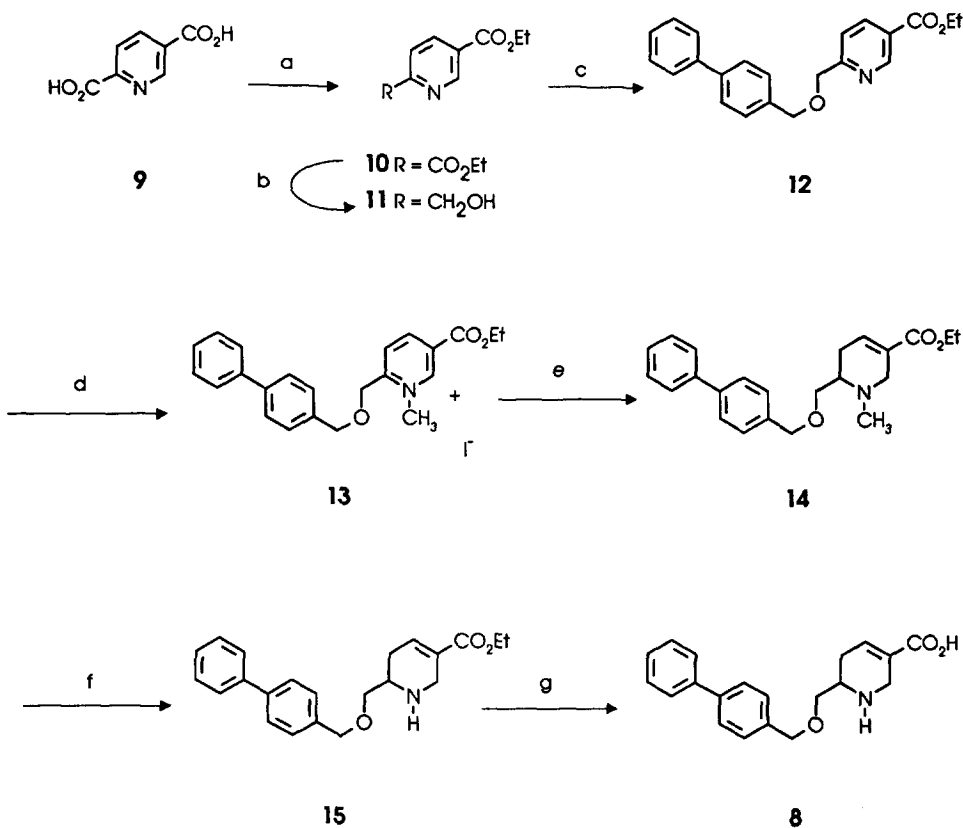
Scheme 1: Synthesis of compound 8. a: \text{H}_2\text{SO}_4 , EtOH, 100%; b: \text{NaBH}_4 , \text{CaCl}_2 , MeOH, 76%; c: \text{NaH} , DMF, 4-diphenyl bromomethane, 79%; d: \text{CH}_3\text{I} , acetonitrile, acetone, 77%; e: \text{NaBH}_4 , MeOH, 43%; f: \alpha -chloroethylchloroformate, \text{CH}_2\text{Cl}_2 , 42%; g: Acetic acid, \text{HCl} gas, 51%
